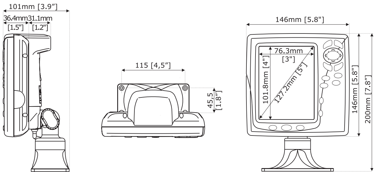
Fig. 7.1 - SKY X5 & COMPACT X5
