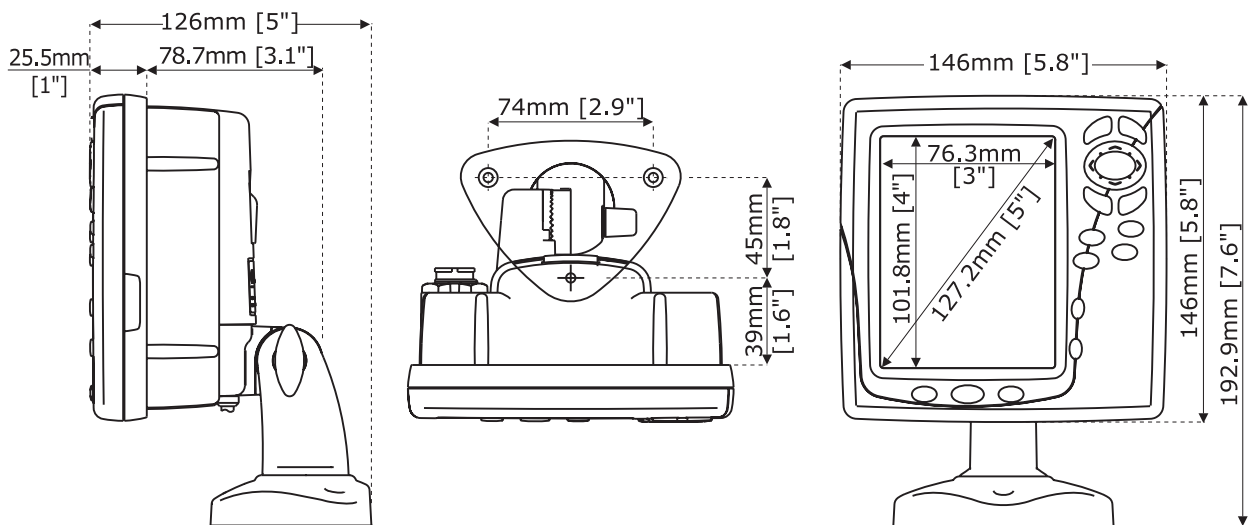
Fig. 7.1a - SKY X5 FISH & COMPACT X5 FISH
