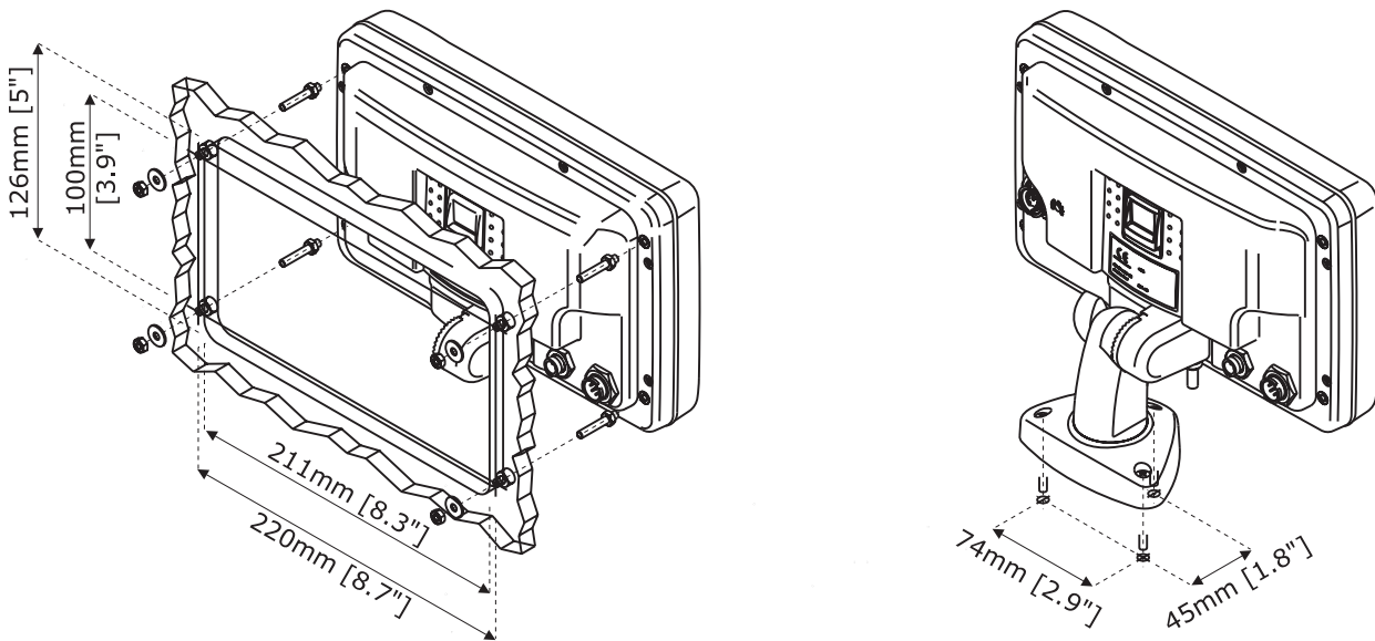
Fig. 7.2a - PANORAMIC 8 HD FISH & COMPACT 8 HD FISH
