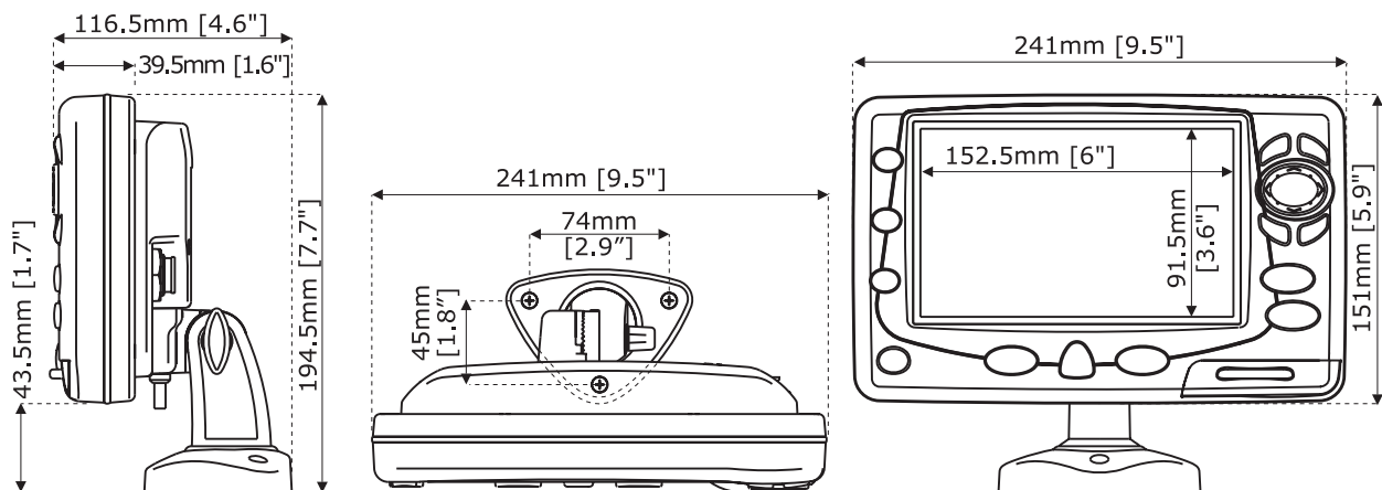
Fig. 7.1a - PANORAMIC 8 HD FISH & COMPACT 8 HD FISH
