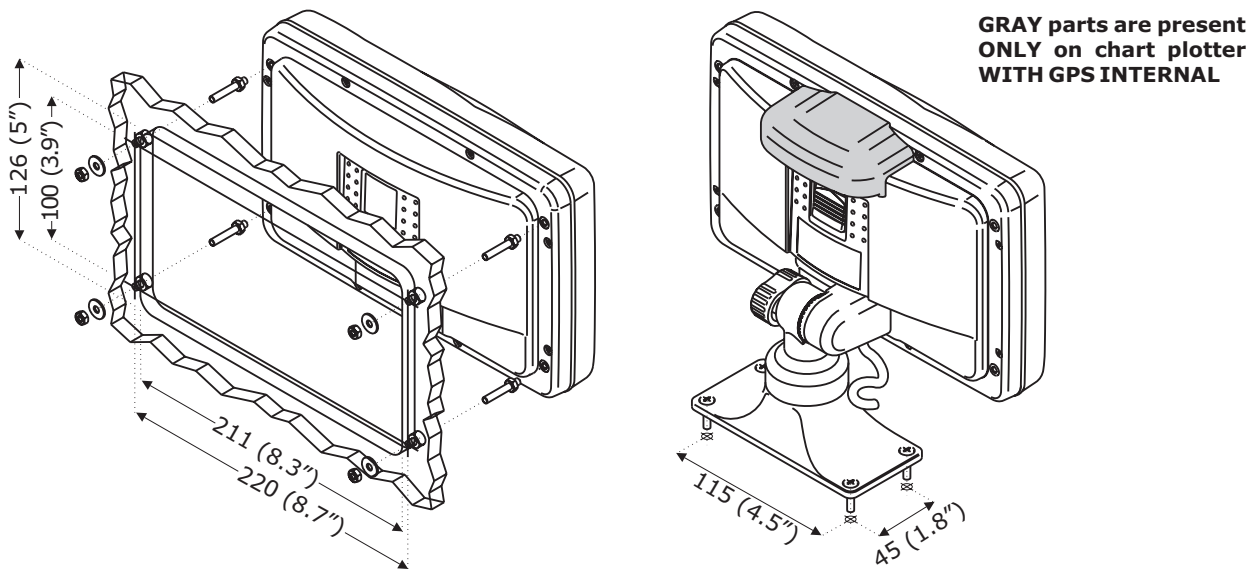
Fig. 7.2 - PANORAMIC 8 XL/HD & COMPACT 8 XL/HD
