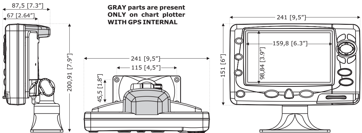
Fig. 7.1 - PANORAMIC 8 XL/HD & COMPACT 8 XL/HD
